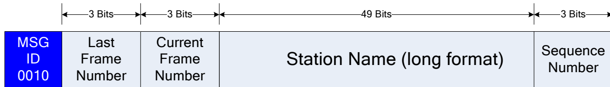
Figure 4-4: Station Name (long format) – Message Structure
