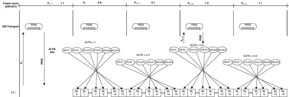
Figure 5-1: Broadcasting ALFN over the HD Radio FM System
