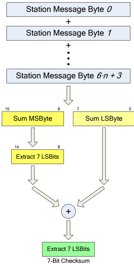
Figure 4-7: Checksum Calculation
