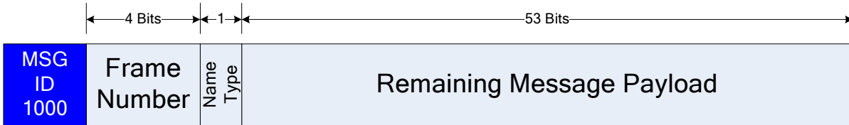
Figure 4-24: General Message Structure for MSG ID 1000
