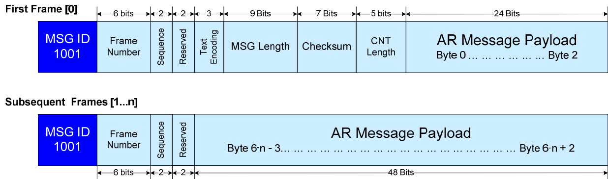
Figure 4-27: Active Radio Message – Message Structure
