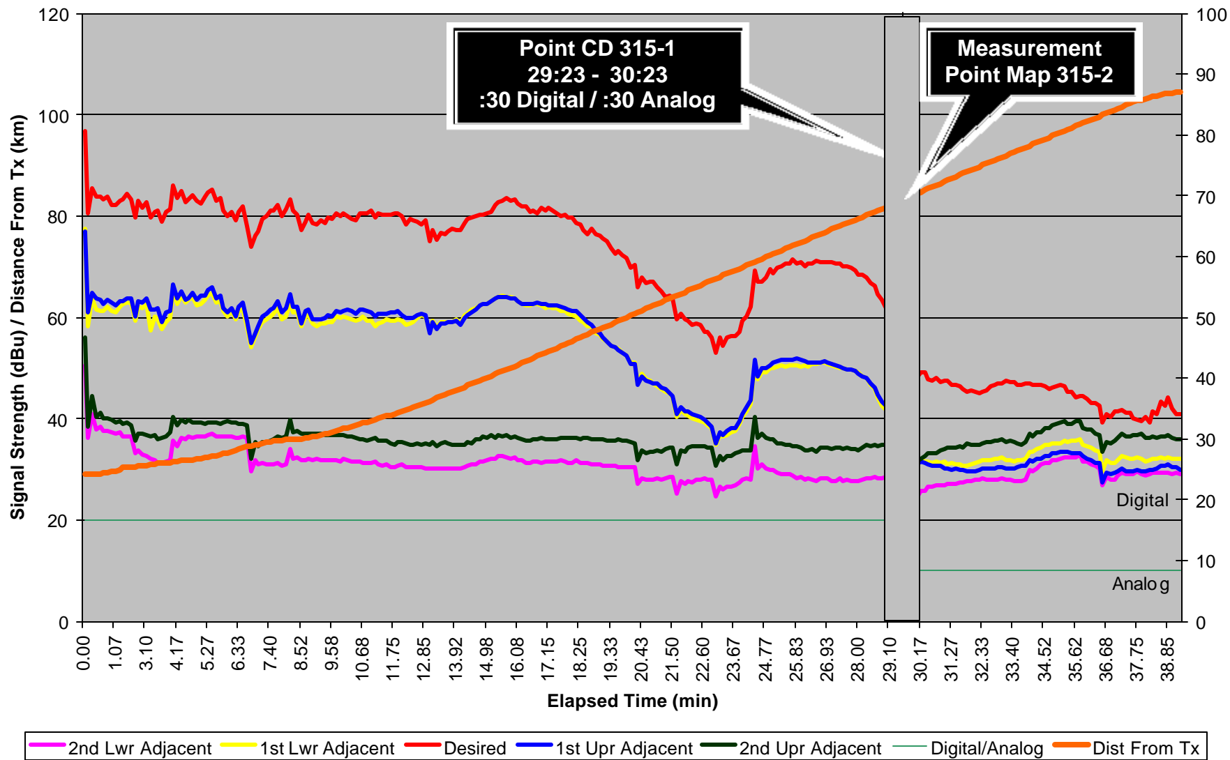
Graph KWNR-315A - KWNR Strip-Chart Recording for Las Vegas 315° Radial
