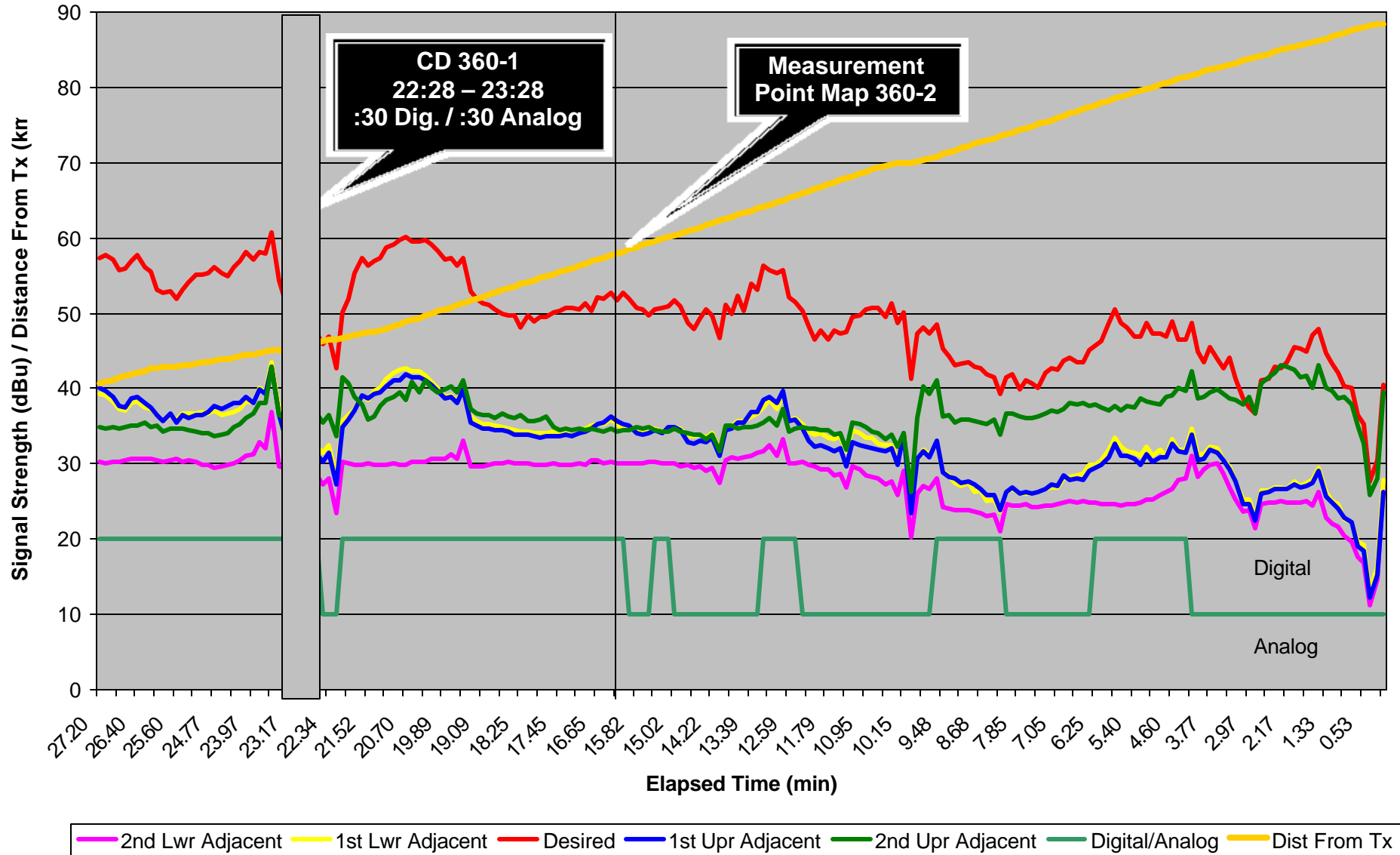
Graph KWNR-360A - KWNR Strip-Chart Recording for Las Vegas 360° Radial
