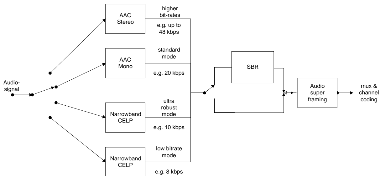
FIGURE 2.2 Source coding overview
