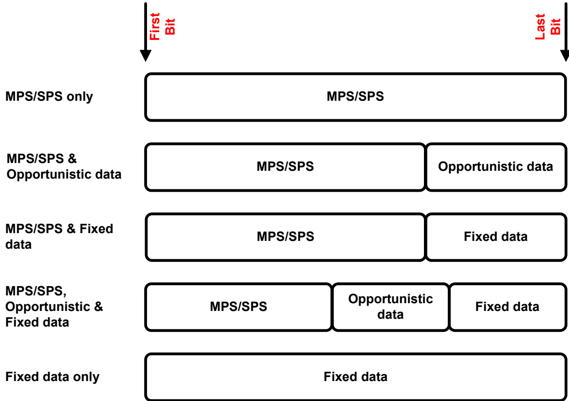
Figure 5-1 L2 PDU structures based on content
