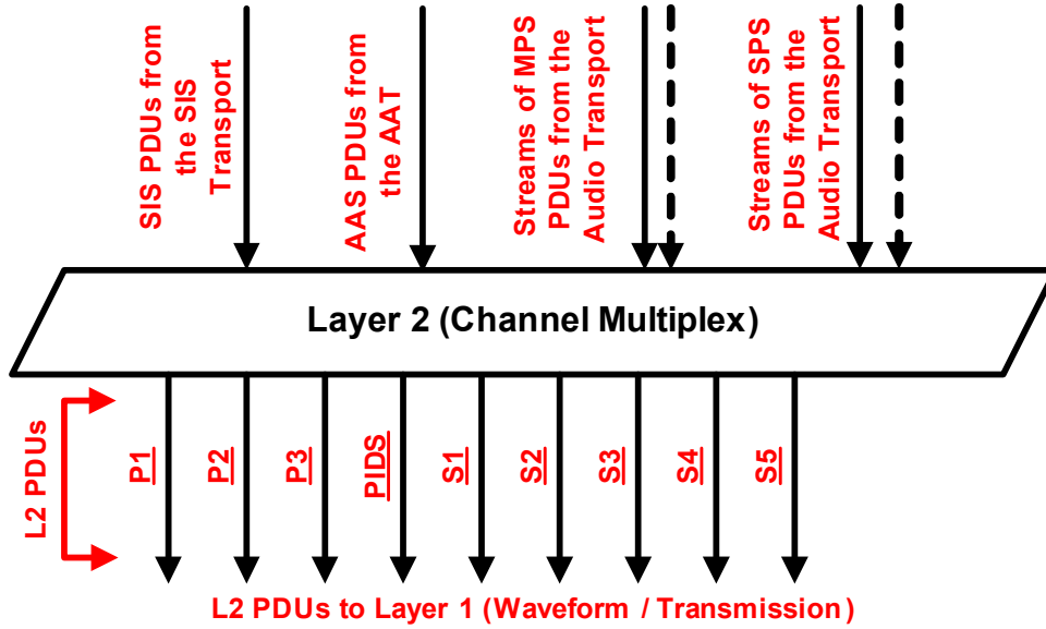
Figure 4-1 Layer 2 - Interface Diagram
