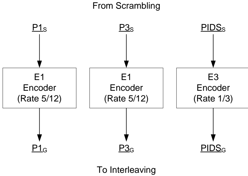
Figure 9-6: Channel Encoding – Service Mode MA3
