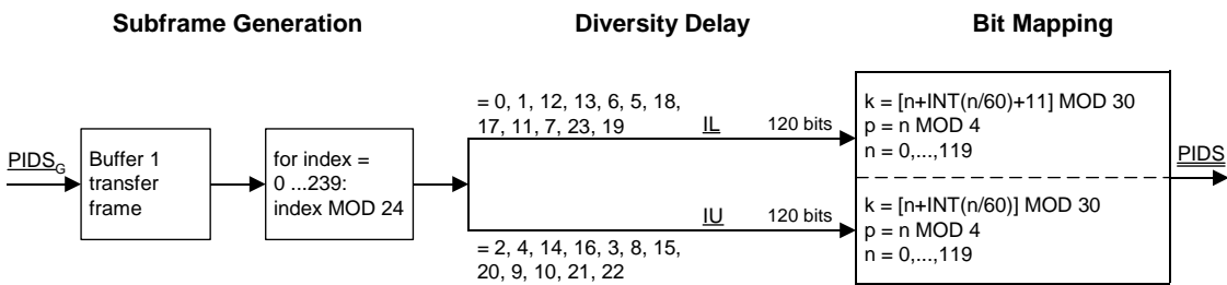
Figure 10-5: PIDS Interleaving Process – All Service Modes
