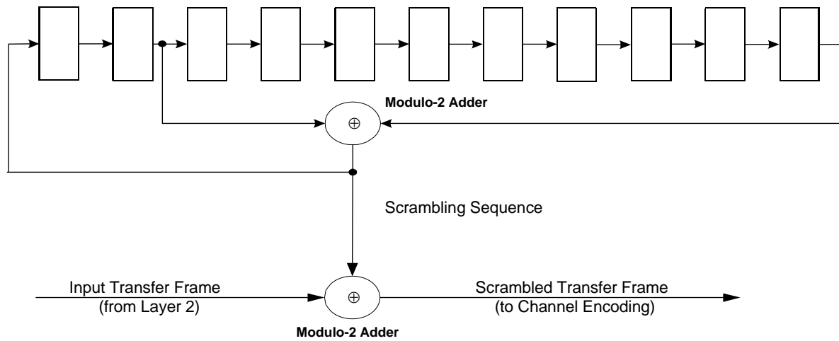
Figure 8-2: Scrambler Block Diagram
