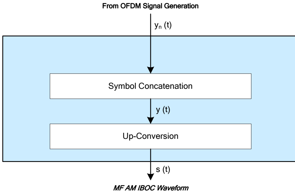
Figure 14-2: All Digital Transmission Subsystem Functional Block Diagram
