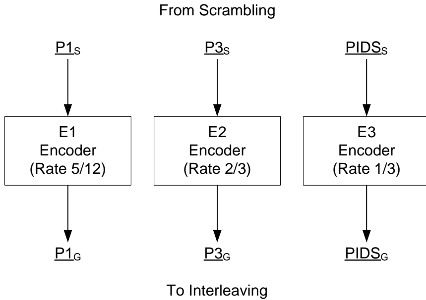
Figure 9-5: Channel Encoding – Service Mode MA1
