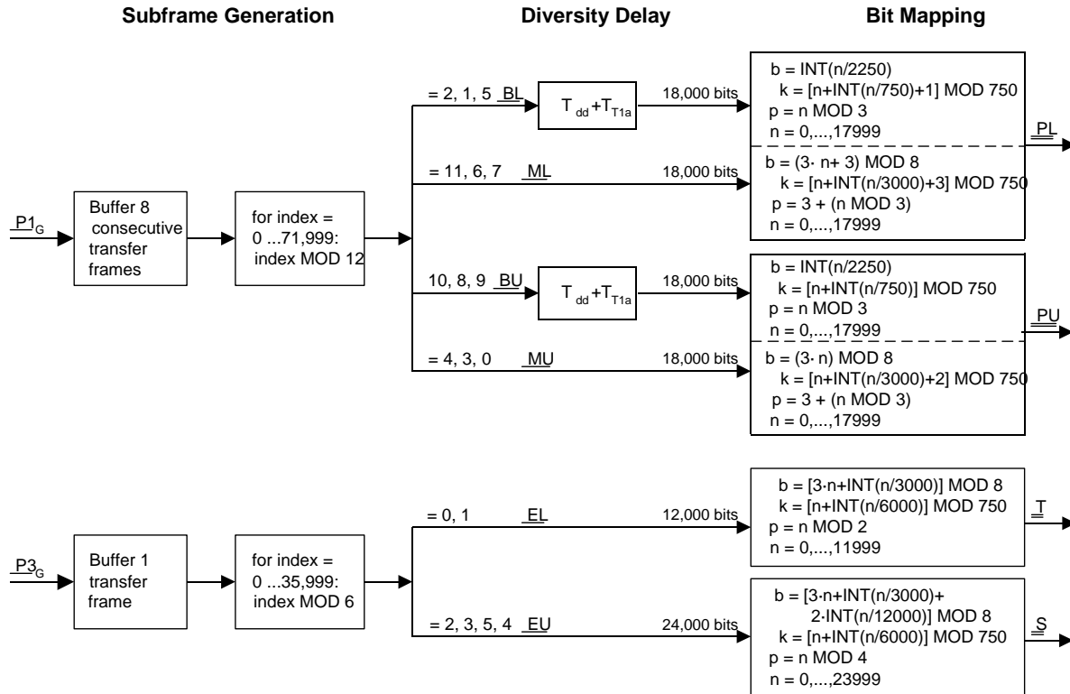
Figure 10-4: Interleaving – Service Mode MA1
