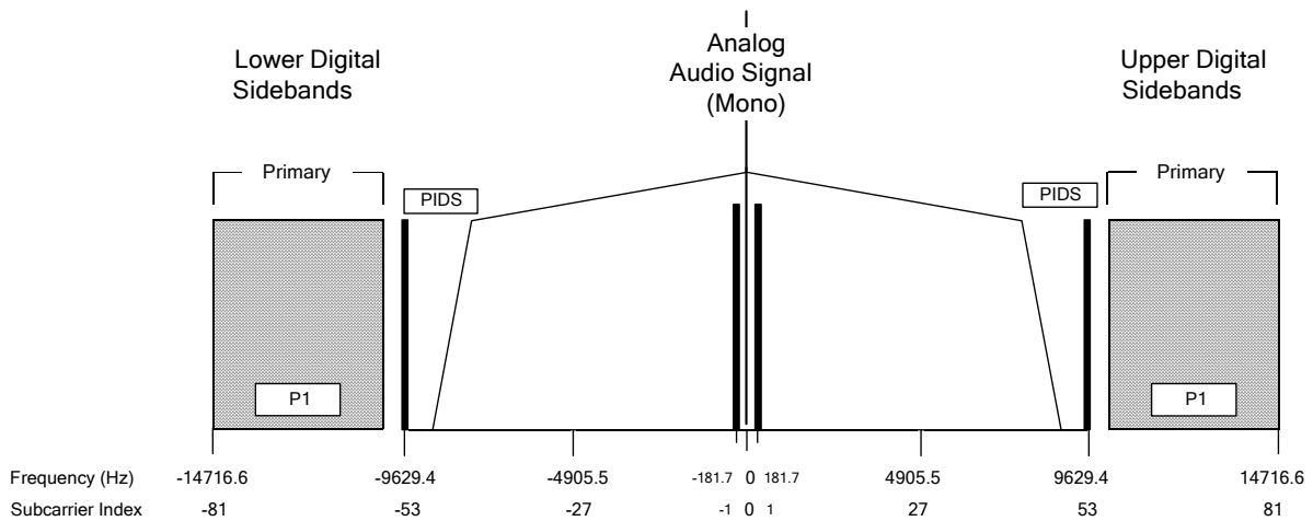
Figure 7-3: Logical Channel Spectral Mapping – Service Mode MA1 (Reduced Digital Bandwidth Configuration)
