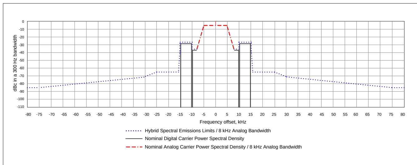
Figure 9. NRSC-5-C hybrid AM IBOC waveform spectral emissions limits for 8 kHz mode analog bandwidth
