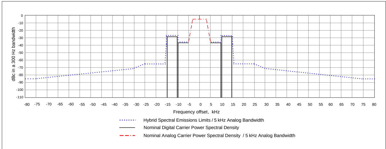
Figure 8. NRSC-5-C hybrid AM IBOC waveform spectral emissions limits for 5 kHz mode analog bandwidth
