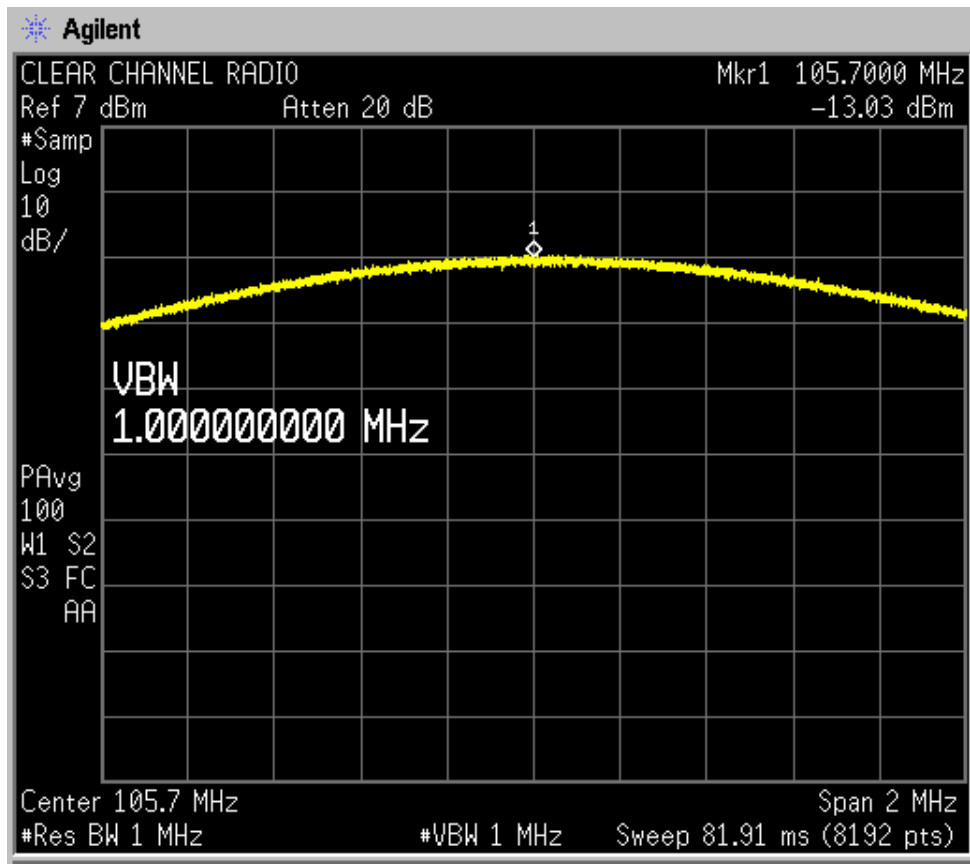
Figure 5 Digital Reference Level Is Observed to Be Certain It Is At the Expected Level with Respect to the Top of the Display
