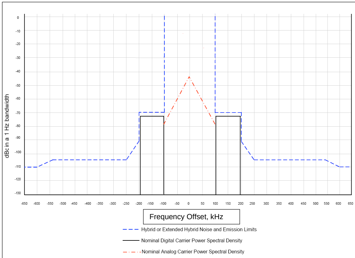
Figure 1 Tractable Specification for Hybrid FM IBOC Power Spectral Density In Decibels with Respect to Analog Carrier Power per Hertz of Bandwidth
