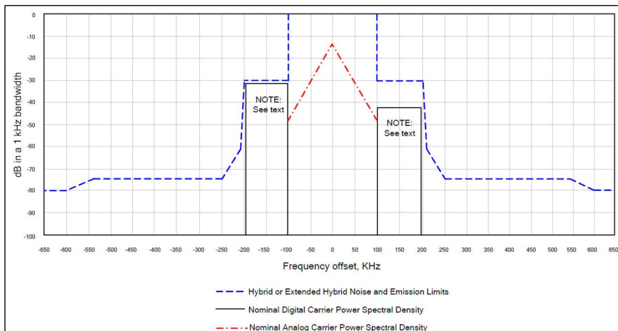
Figure 1. NRSC-5-C hybrid FM IBOC waveform noise and emission limits
