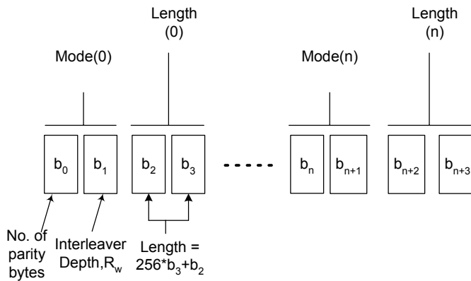
Figure 7-3 Mode bit definitions
