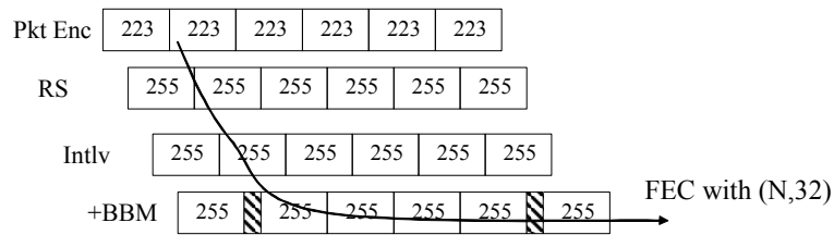
Figure 7-4 Fixed Sub-Channel Byte Stream
