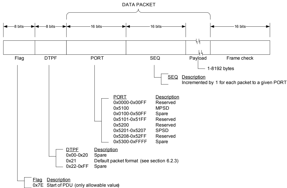
Figure 6-2 AAS PDU Structure
