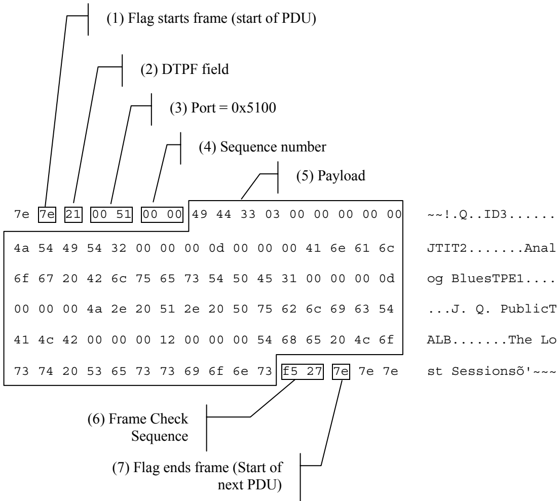
Figure 6-3 Encapsulated Packet – Example
