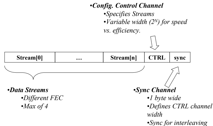
Figure 7-2 Fixed Bearer Channel Structure
