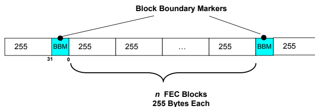
Figure 6-6 FEC Blocking with Block Boundary Markers
