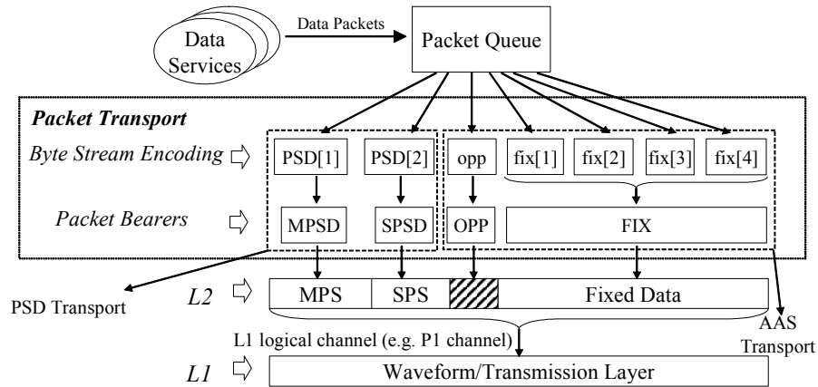
Figure 4-2 HD RLS Packet Transport Mechanism
