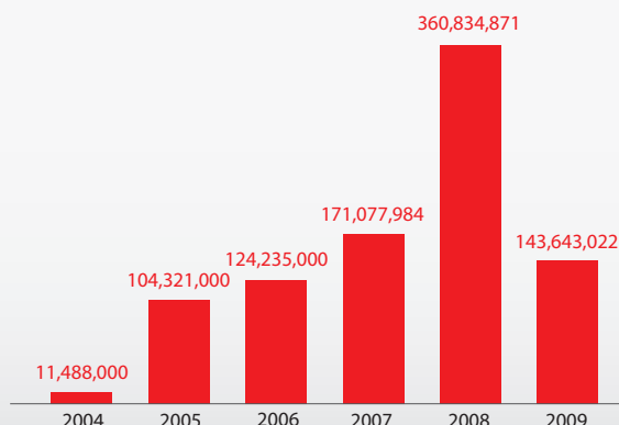
Figure 29. Number of records compromised per year in breaches investigated by Verizon and the United States Secret Service
