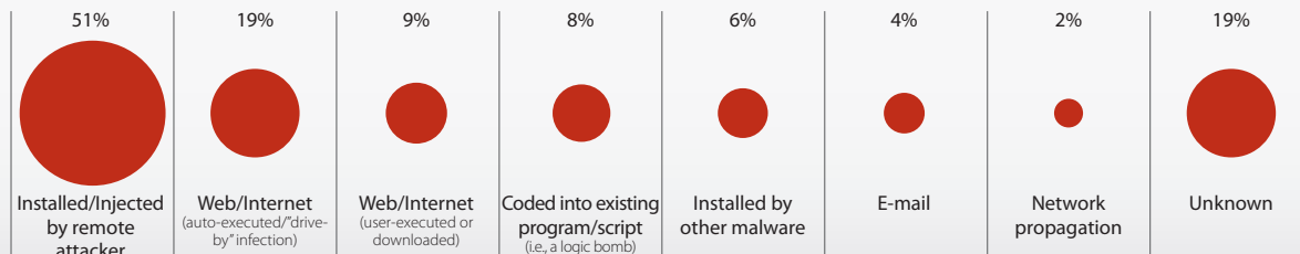
Figure 18. Malware infection vectors by percent of breaches within Malware
